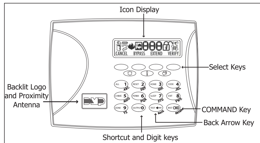
Thinline™ Series Icon Keypad
